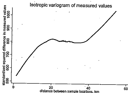
Figure 10. Standardized isotropic variogram of measured mCi/km 2 .
