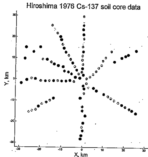
Figure 9. Plot of measured mCi/km 2 (marker color) vs. location.
