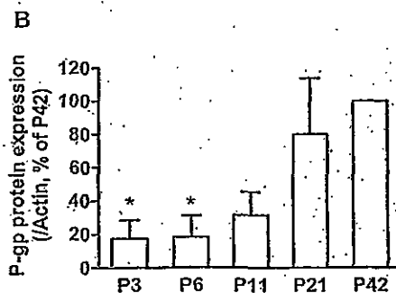
FIG. 6. Ontogenetic expression of P-gp protein in the crude membrane fractions of cerebral cortex from P3 through 42 rats. A, crude membrane fractions were prepared from the cerebral cortex from P3 to 42 rats. Each sample (50 \mu g protein/lane) was subjected to SDS-polyacrylamide gel electrophoresis (8.5% separating gel). P-gp and actin proteins were detected by monoclonal anti-P-gp C219 antibody and monoclonal antiactin antibody, respectively. A typical immunoblot is shown in A. B, the intensities of the bands of P-gp and actin were quantified by densitometric analysis. For P-gp, the intensity of the upper band was used for the calculation. The bar represents the ratio of the band densities of P-gp and actin relative to that in P42 rats. Each bar represents the mean \pm S.E. of three determinations using three crude membrane fractions of the cerebral cortex prepared independently from one to four rats. Asterisks represent statistically significant differences toward P42 rats; *, P < 0.05 .
