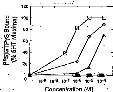
Fig. 3. Representative Concentration-Response Curves for [ 3 S]GTPγS Binding by Tamiflu and GS4071 in the Rat Whole Brain Membranes
