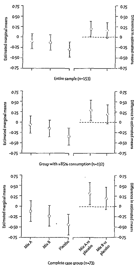
Figure 3: Estimated marginal means by challenge type and difference in estimated means in GHA under model 2 for 3-year-old children. Bars=95% CI. Dashed line=zero difference between mean GHA under active mix and mean GHA under placebo.
