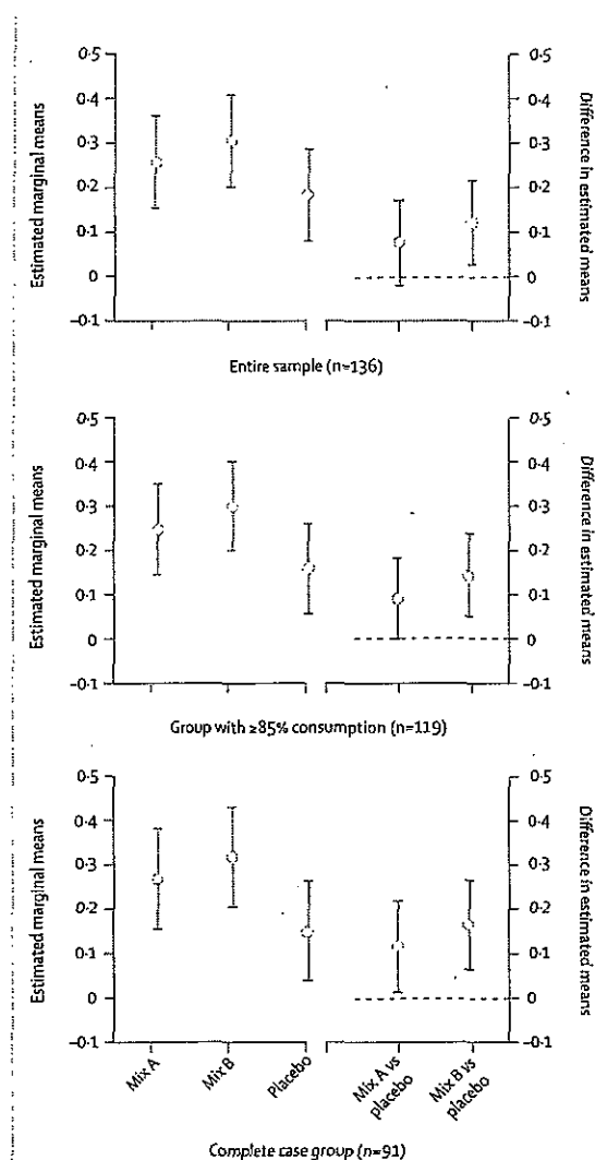
Figure 4: Estimated marginal means by challenge type and difference in estimated means in GHA under model 2 for 8/9-year-old children. Bars=95% CI. Dashed line=zero difference between mean GHA under active mix and mean GHA under placebo.
