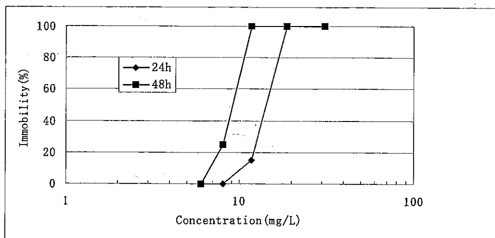
Figure 1 Concentration-Response (Immobilty) Curve
