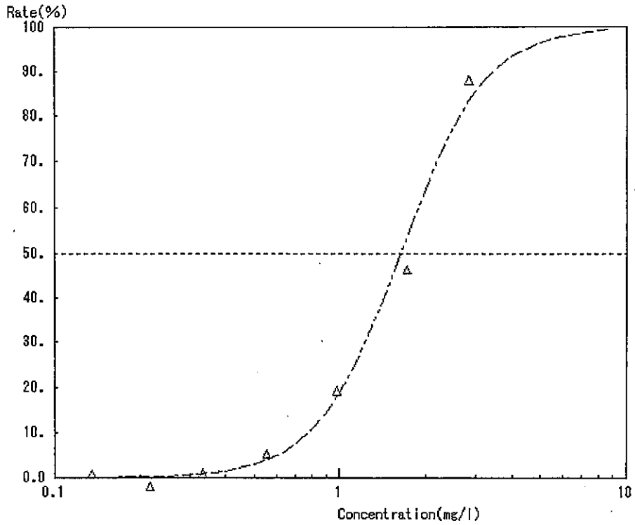
Dose-response curve for EC50 of Algae Growth Test (Logit method) 132650
