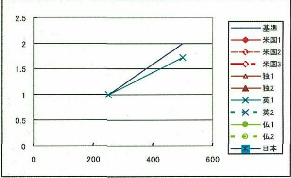
54 Mefenamic acid 0 0
