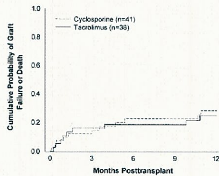
Figure 3. Kaplan-Meier plot for time to graft failure or death. Log-rank comparison of treatment groups, P = .789 .
