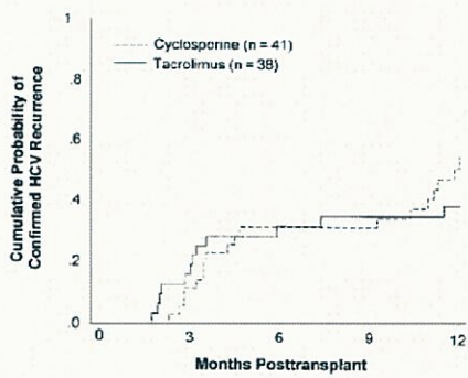
Figure 1. Kaplan-Meier plot for time to HCV recurrence confirmed by biopsy. Log-rank comparison of treatment groups, P = .19 .
