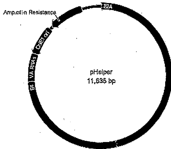
図6 pHelper
