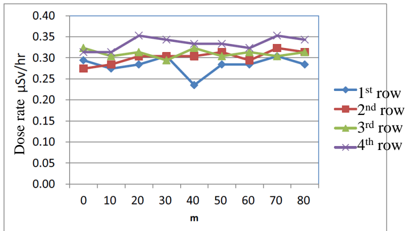
Ambient dose rate at 1 m above the ground surface
