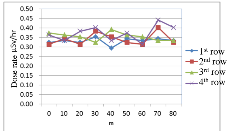
Ambient dose rate at 10cm above the ground surface
