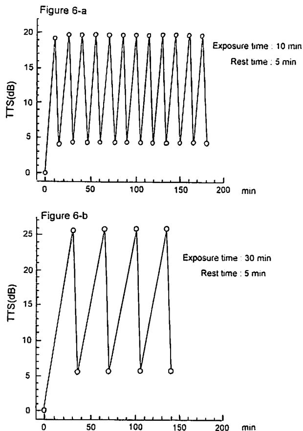
Fig. 6. Prediction TTS values for short rest time
