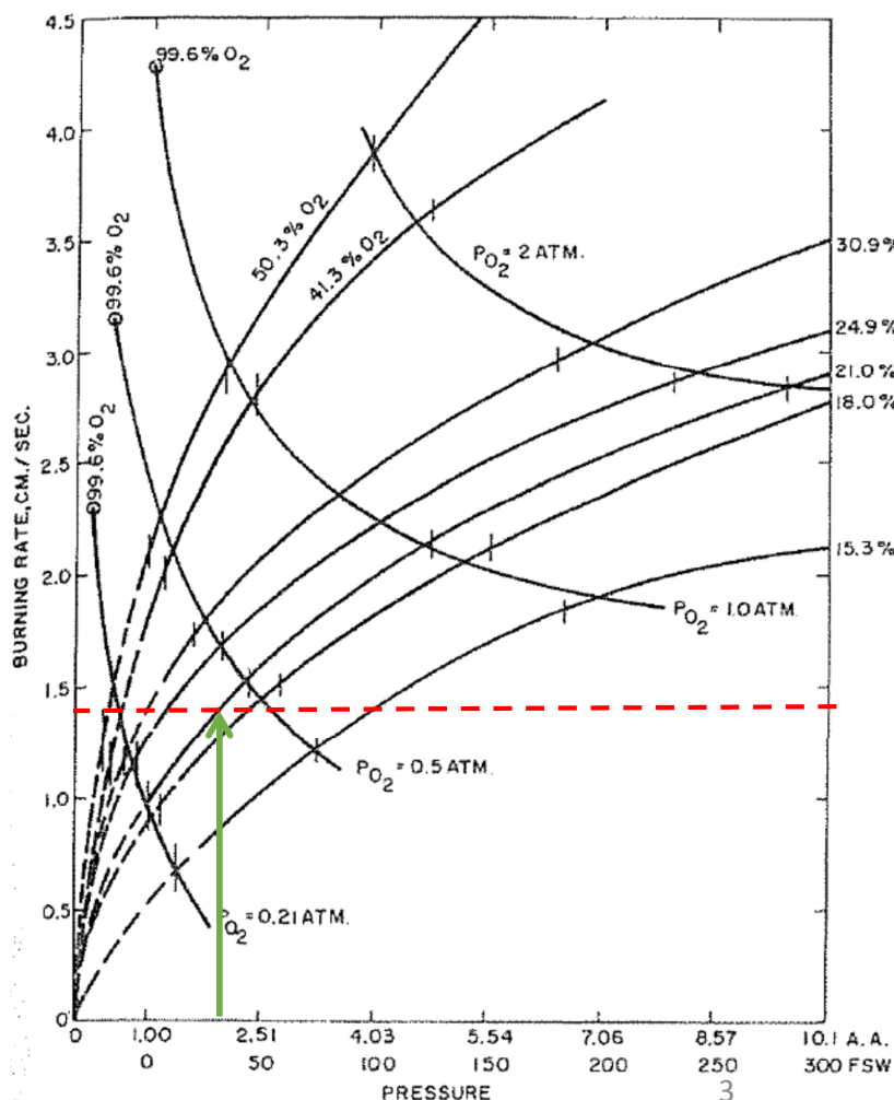
J.Fire&FlammabilityVol.1p.91 Fig.1
