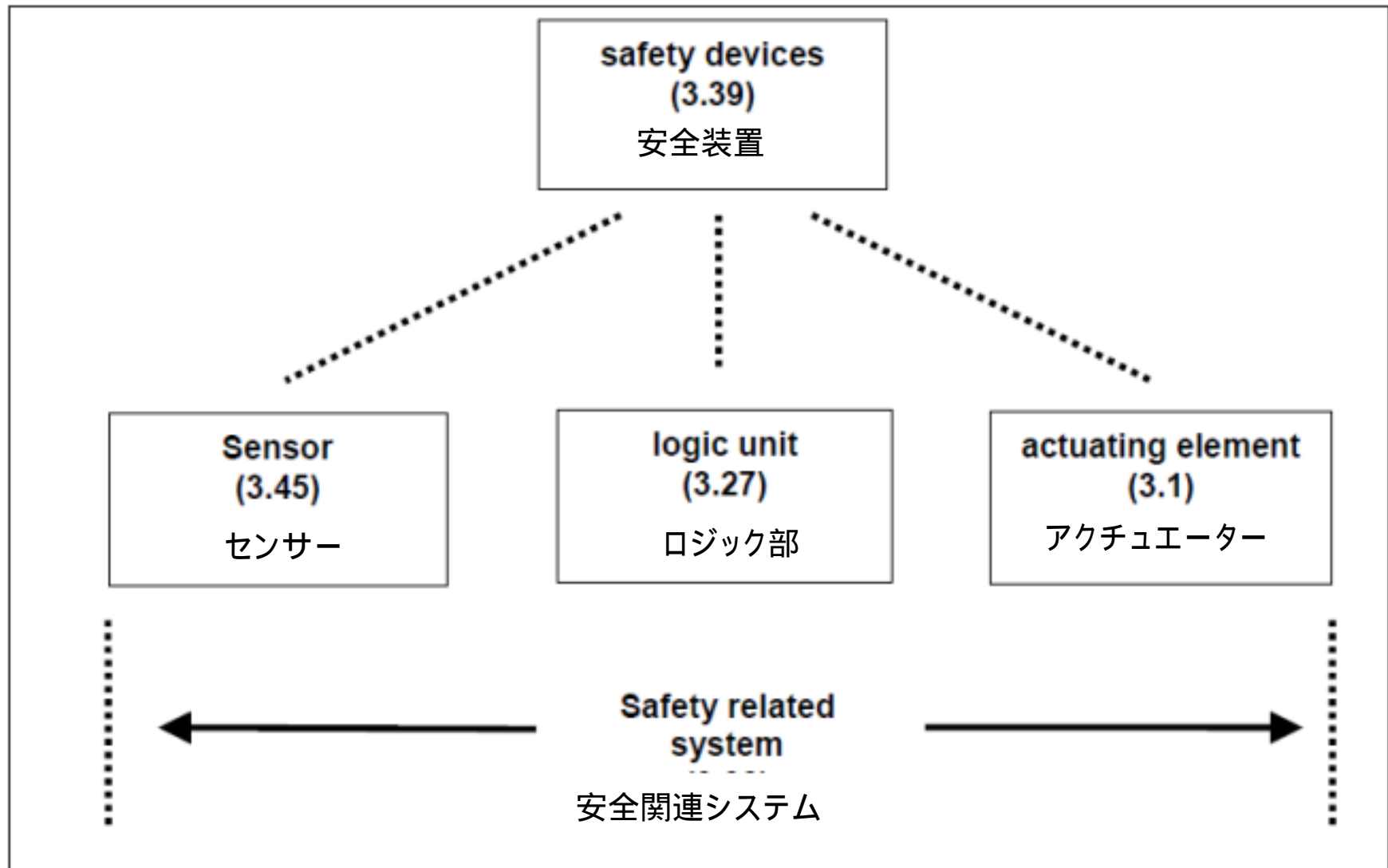
Figure 4 – Definition and components of a safety-related system
