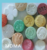
MDMA
