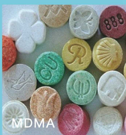
MDMA
