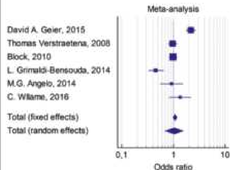
Fig. 2. Forest plot,
