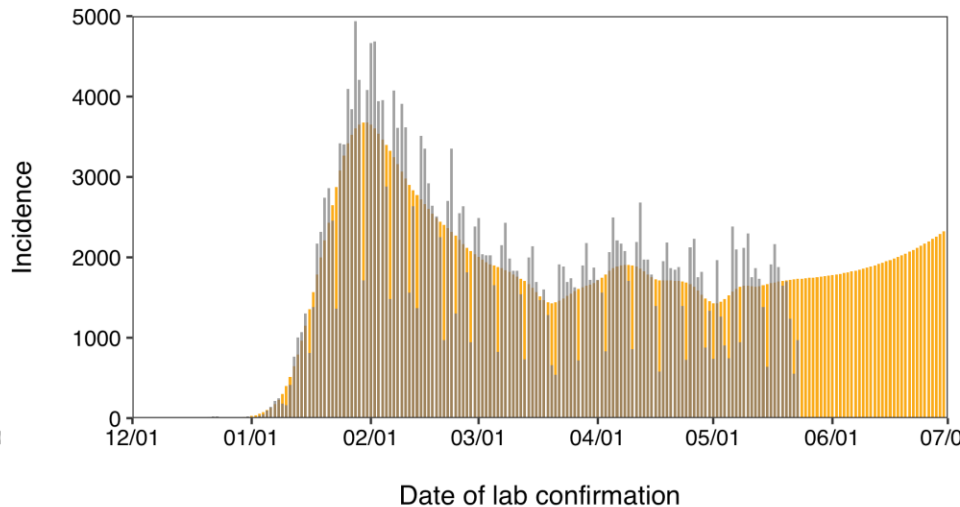
Fukuoka ensemble
