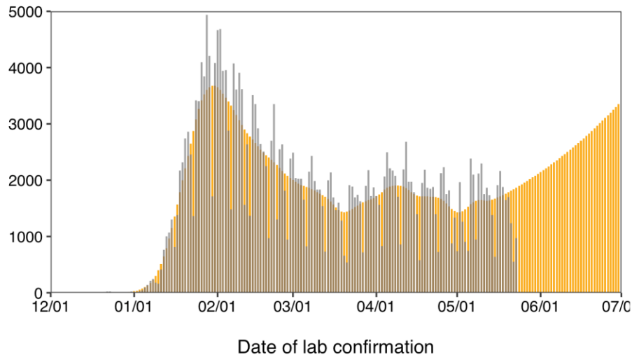
Fukuoka autoregression
